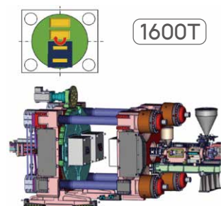
Molding with vertical turntable
