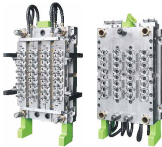
32 cavities
