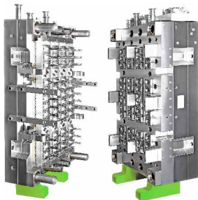
48cavities
