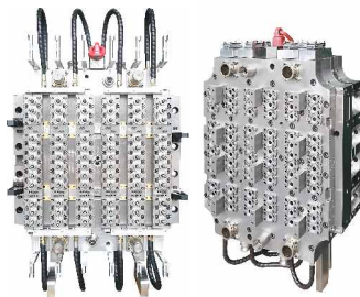
72 cavities
